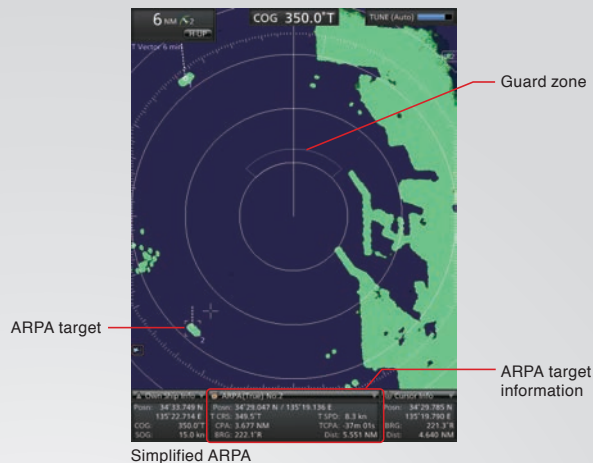
Simplified ARPA
